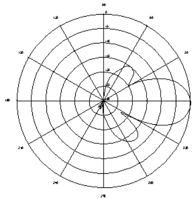
RF Patterns Horizontal Cut, typ.
