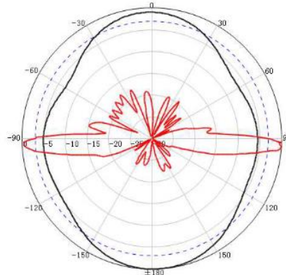
V-Pol @ 2450MHz
